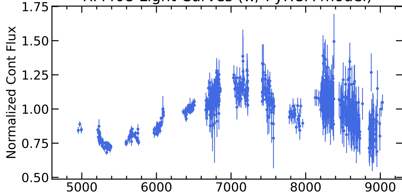
RM408 Light Curves (w/ PyROA model)
