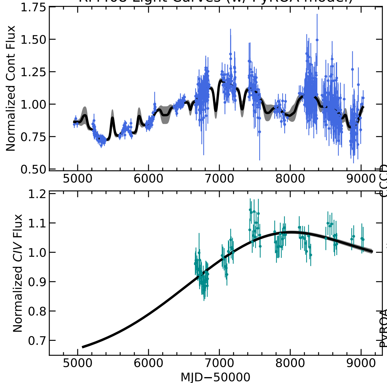
RM408 Light Curves (w/ PyROA model)
