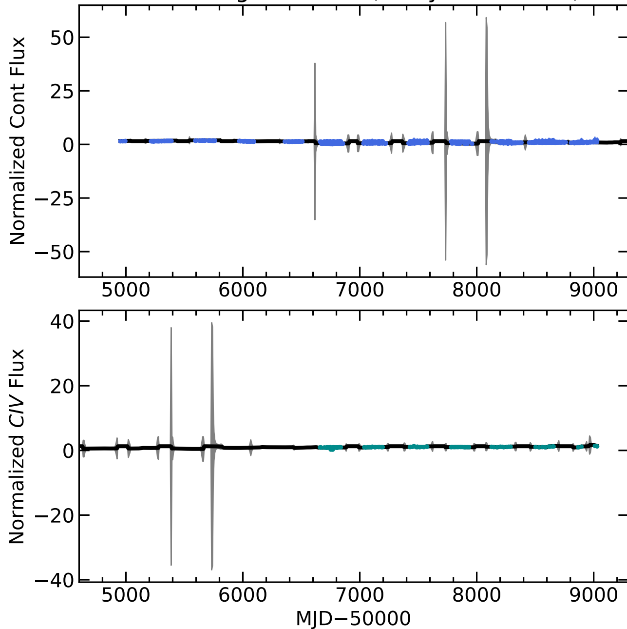
RM409 Light Curves (w/ PyROA model)
