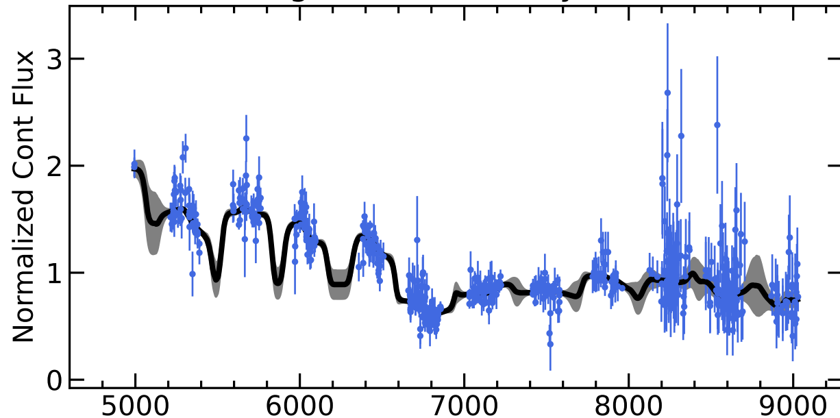
RM411 Light Curves (w/ PyROA model)
