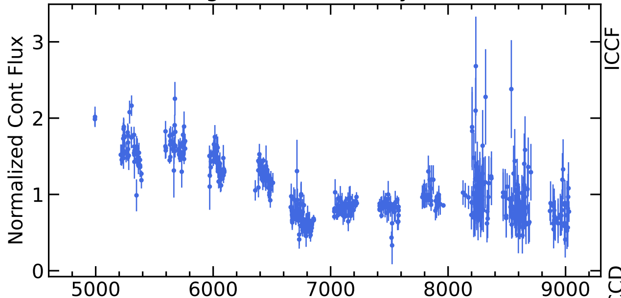
RM411 Light Curves (w/ PyROA model)
