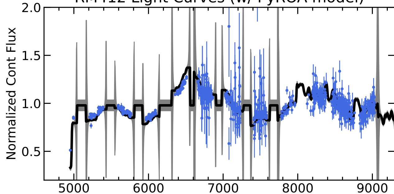
RM412 Light Curves (w/ PyROA model)
