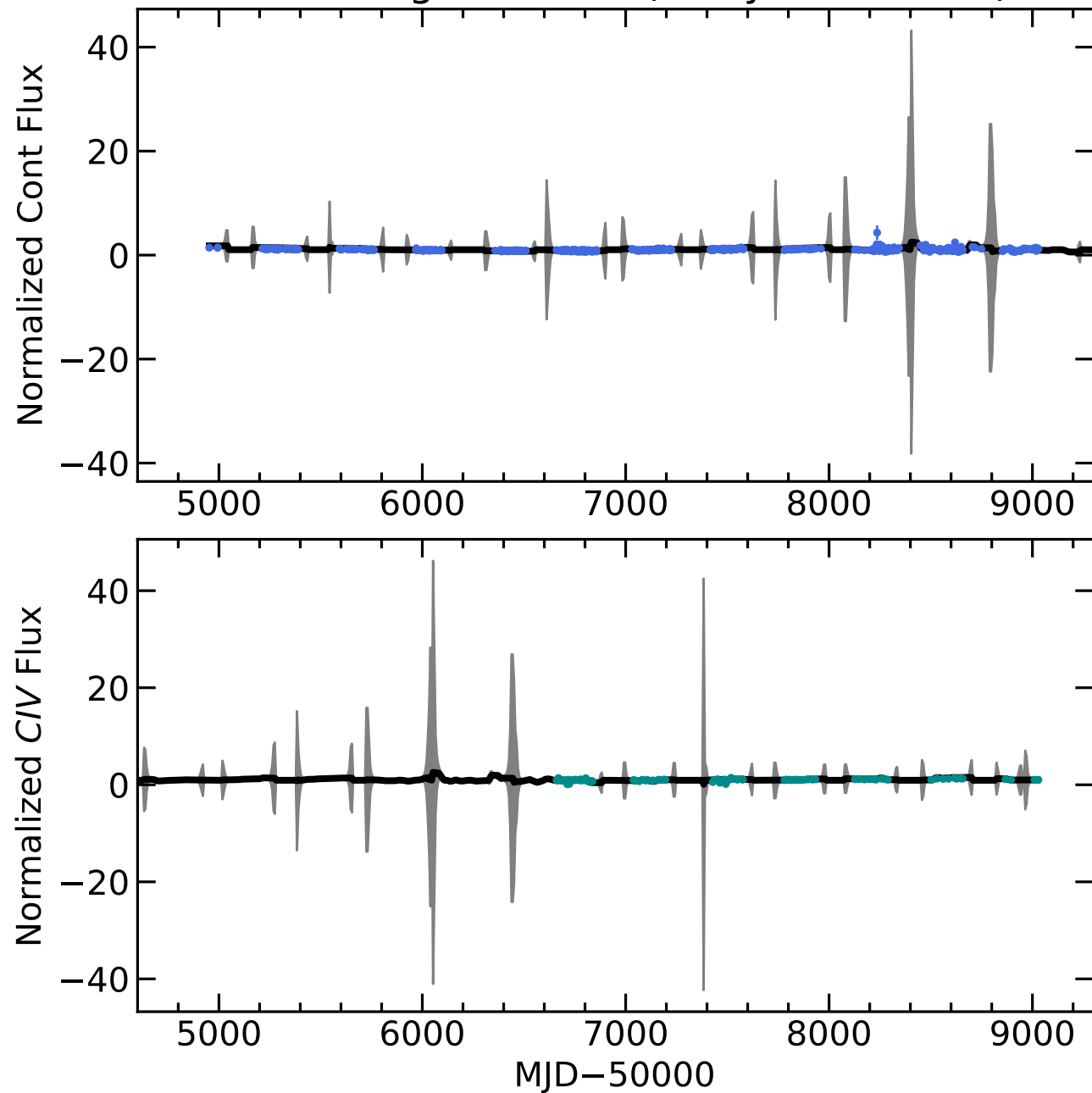
RM413 Light Curves (w/ PyROA model)
