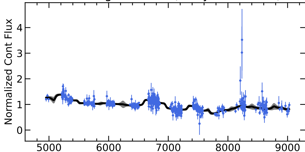
RM415 Light Curves (w/ PyROA model)
