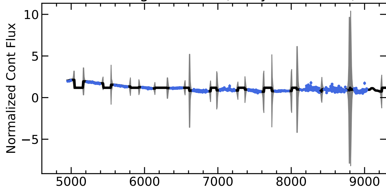
RM416 Light Curves (w/ PyROA model)
