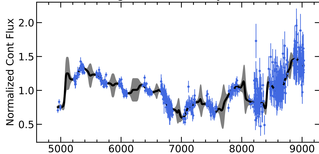
RM418 Light Curves (w/ PyROA model)
