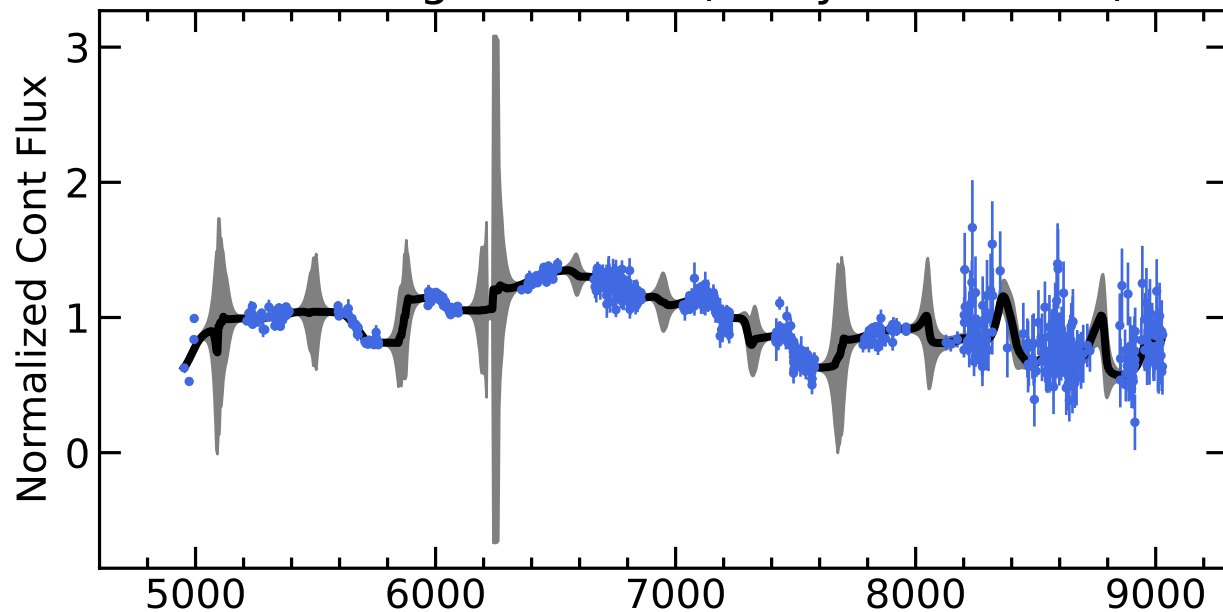
RM419 Light Curves (w/ PyROA model)
