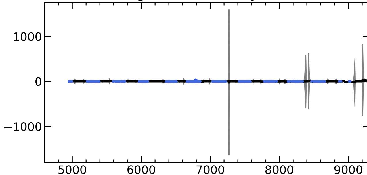
RM420 Light Curves (w/ PyROA model)
