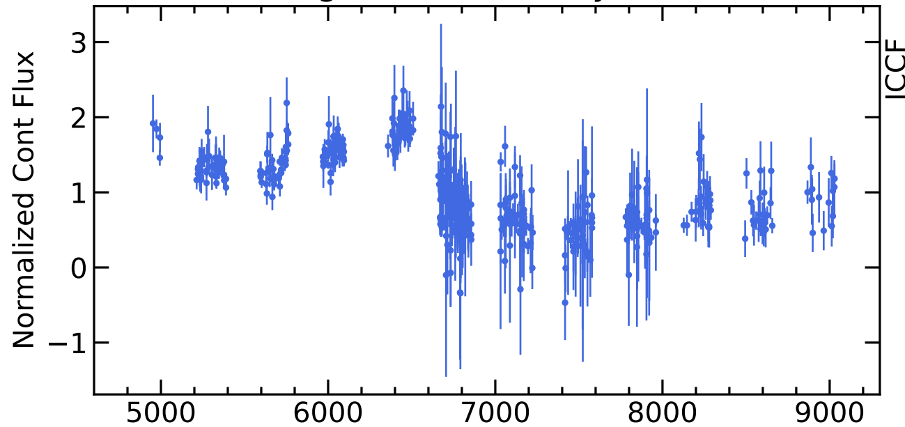
RM421 Light Curves (w/ PyROA model)
