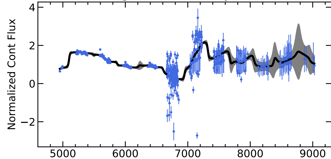
RM422 Light Curves (w/ PyROA model)
