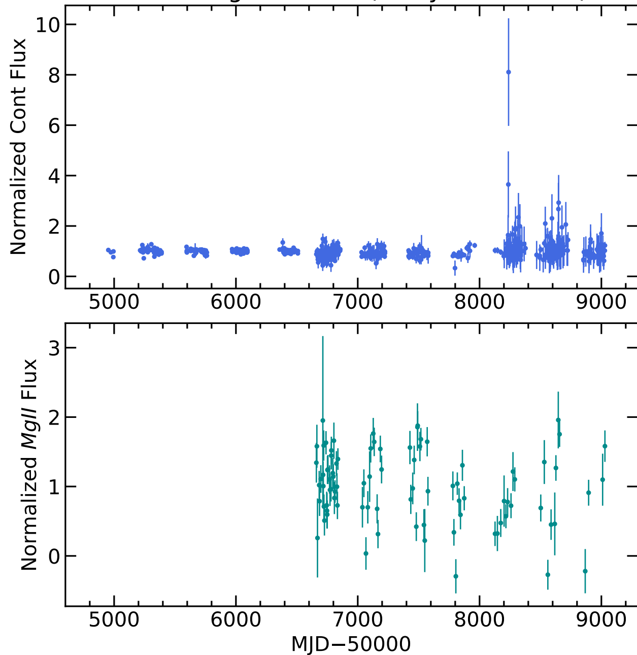
RM425 Light Curves (w/ PyROA model)
