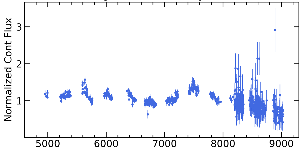
RM426 Light Curves (w/ PyROA model)
