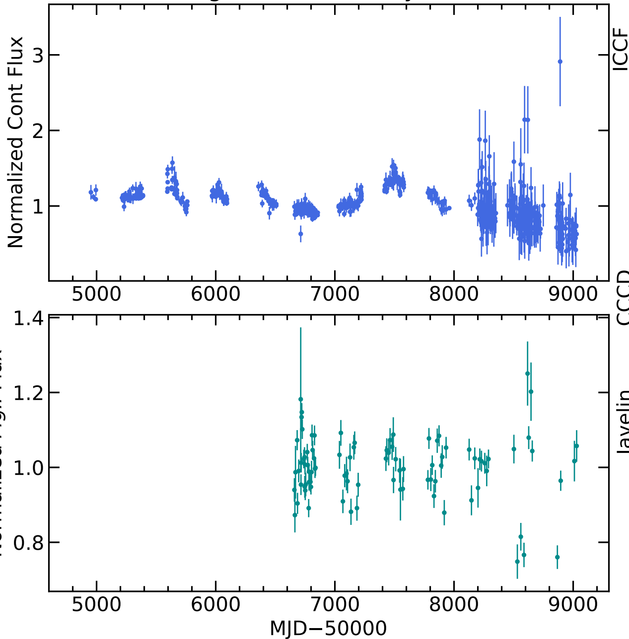
RM426 Light Curves (w/ PyROA model)
