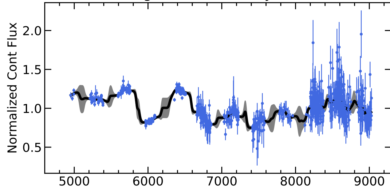
RM427 Light Curves (w/ PyROA model)
