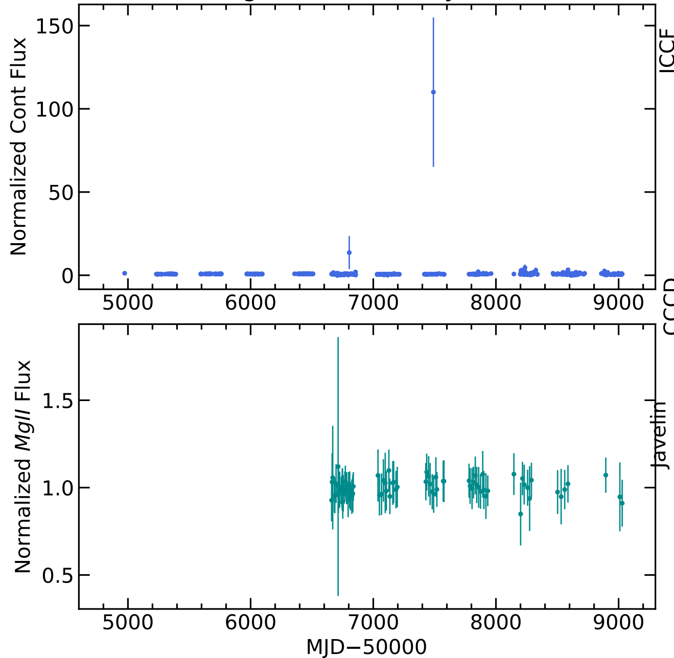
RM429 Light Curves (w/ PyROA model)
