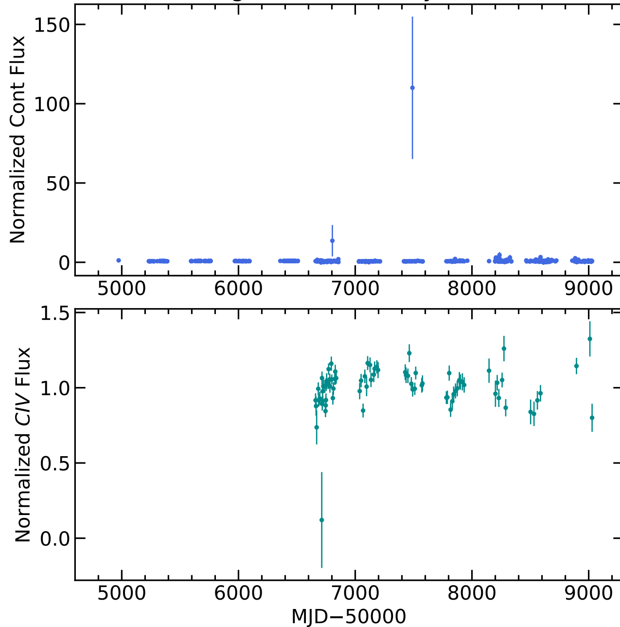
RM429 Light Curves (w/ PyROA model)
