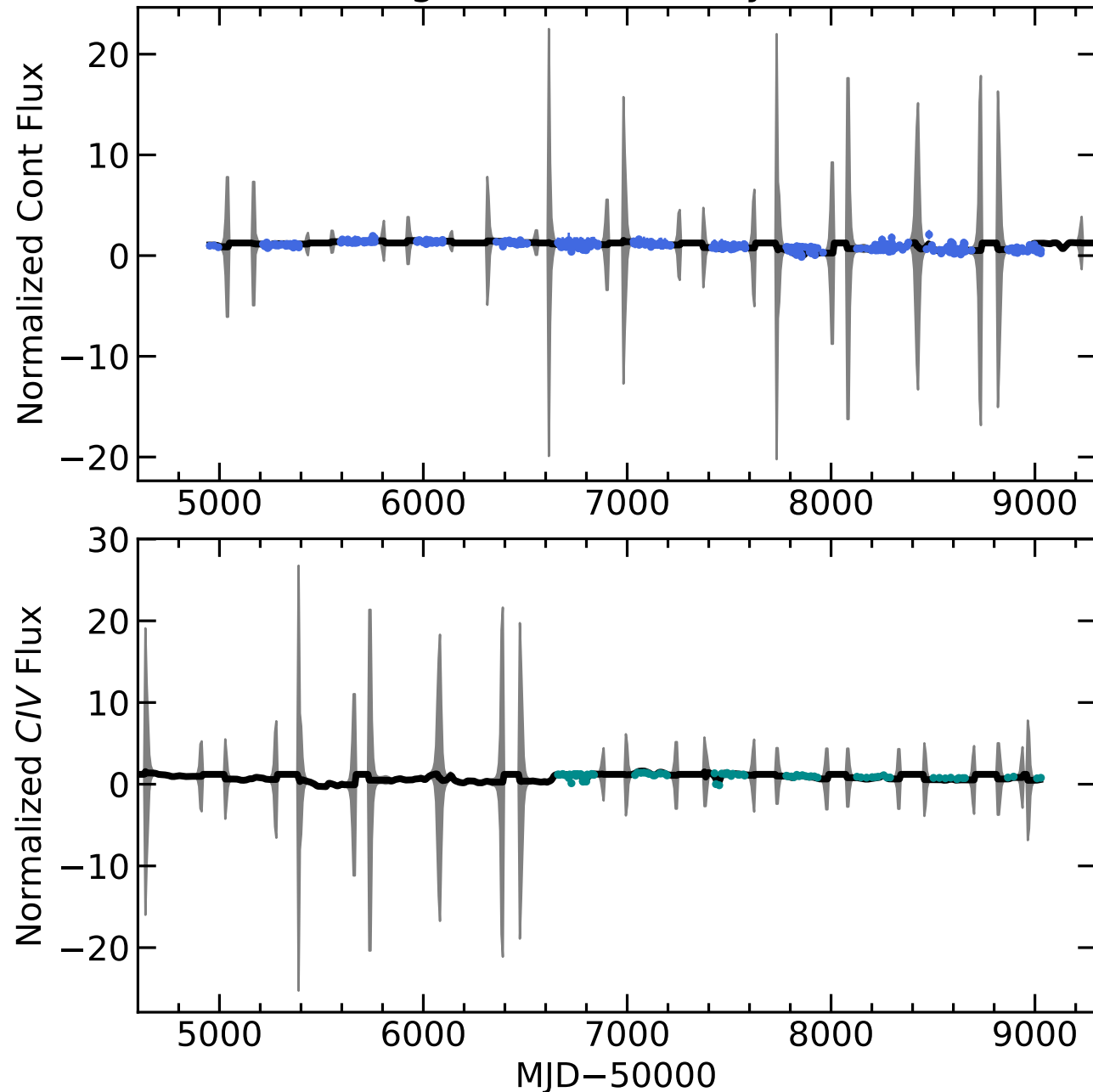
RM430 Light Curves (w/ PyROA model)
