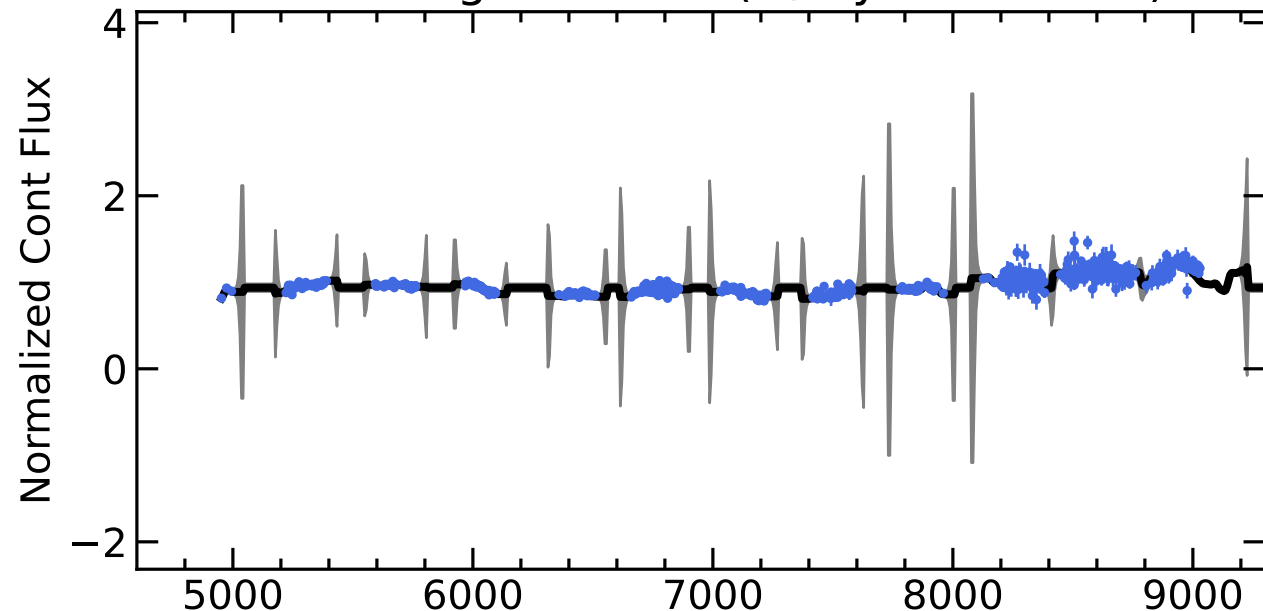
RM431 Light Curves (w/ PyROA model)
