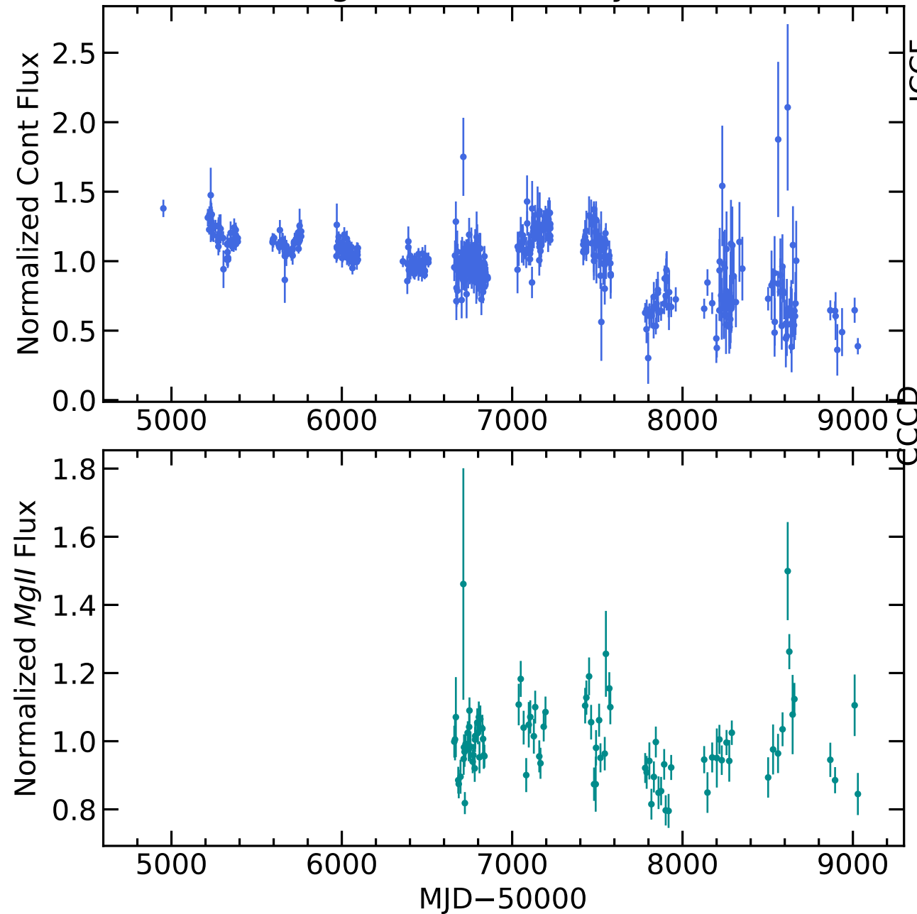
RM433 Light Curves (w/ PyROA model)
