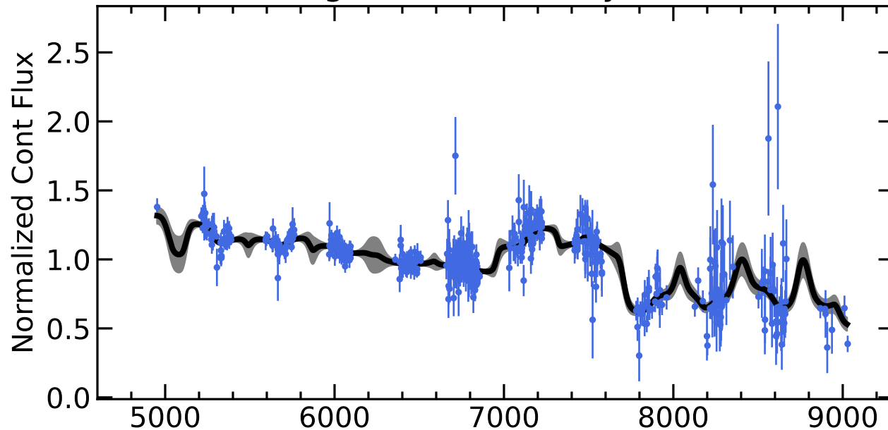
RM433 Light Curves (w/ PyROA model)
