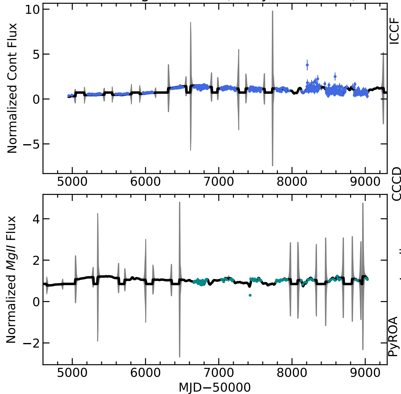
RM434 Light Curves (w/ PyROA model)
