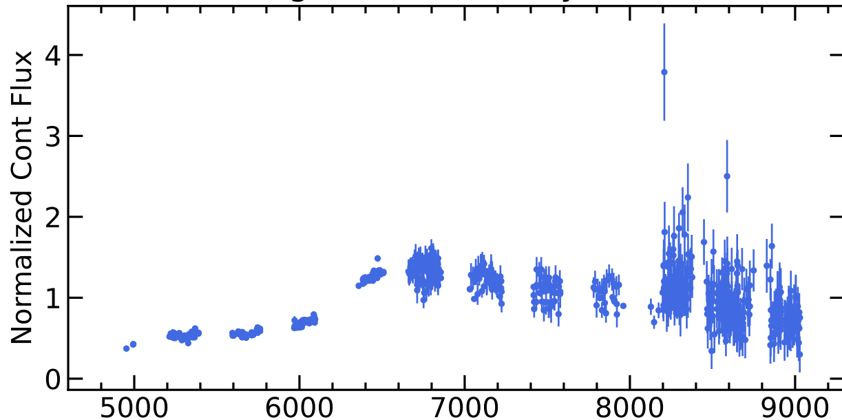
RM434 Light Curves (w/ PyROA model)
