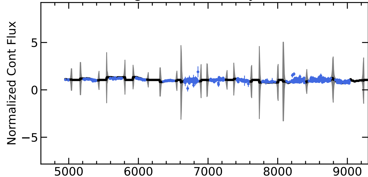
RM435 Light Curves (w/ PyROA model)
