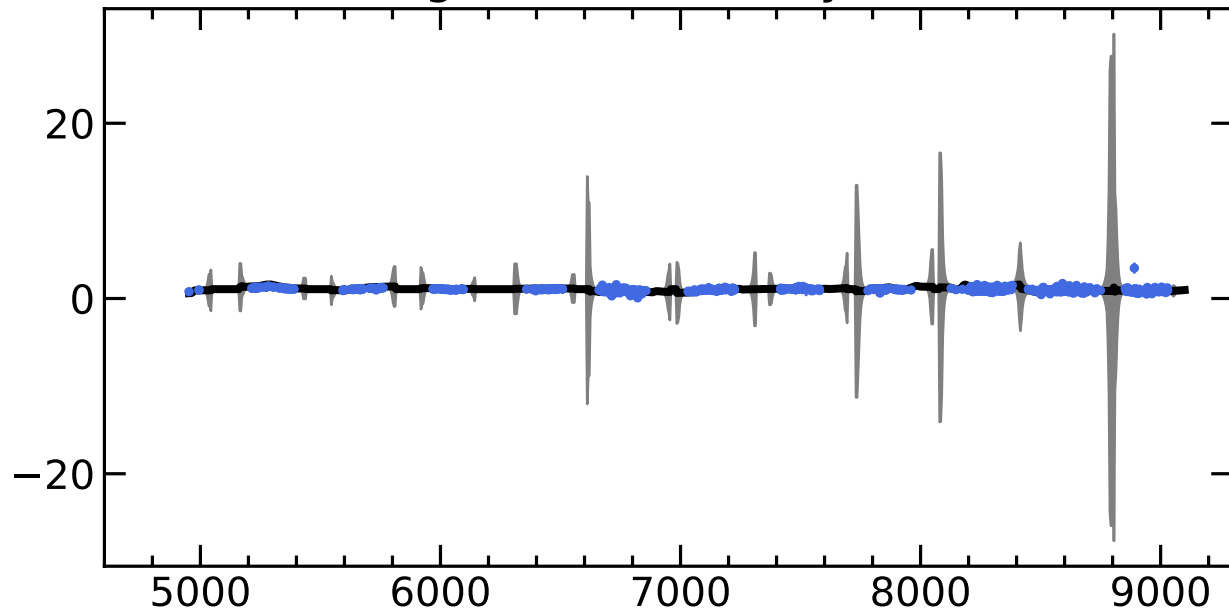
RM436 Light Curves (w/ PyROA model)
