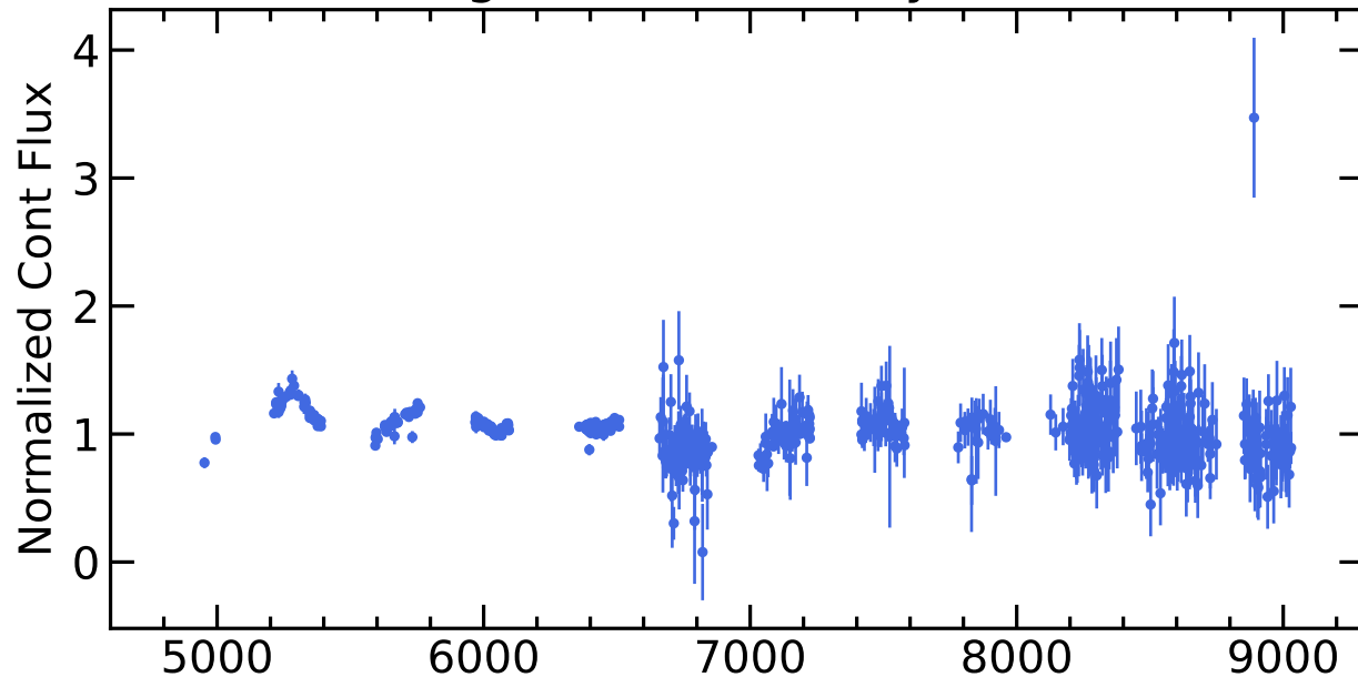
RM436 Light Curves (w/ PyROA model)
