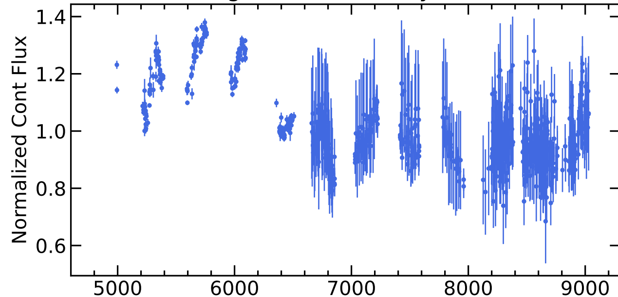
RM437 Light Curves (w/ PyROA model)
