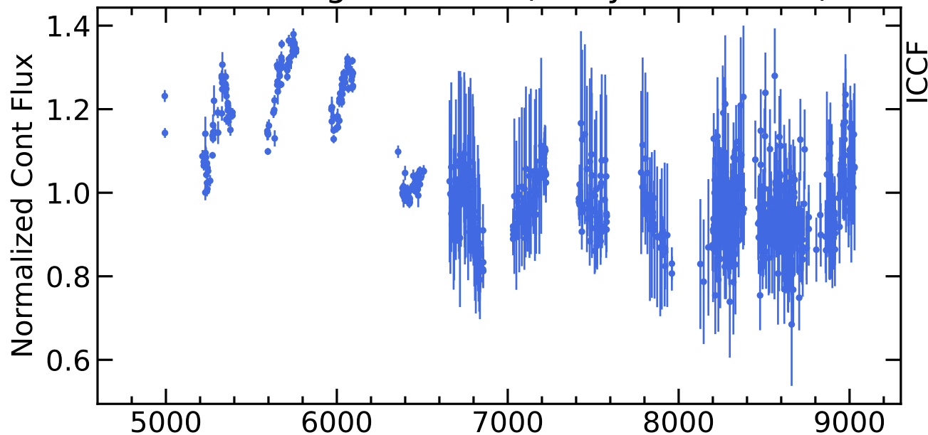
RM437 Light Curves (w/ PyROA model)
