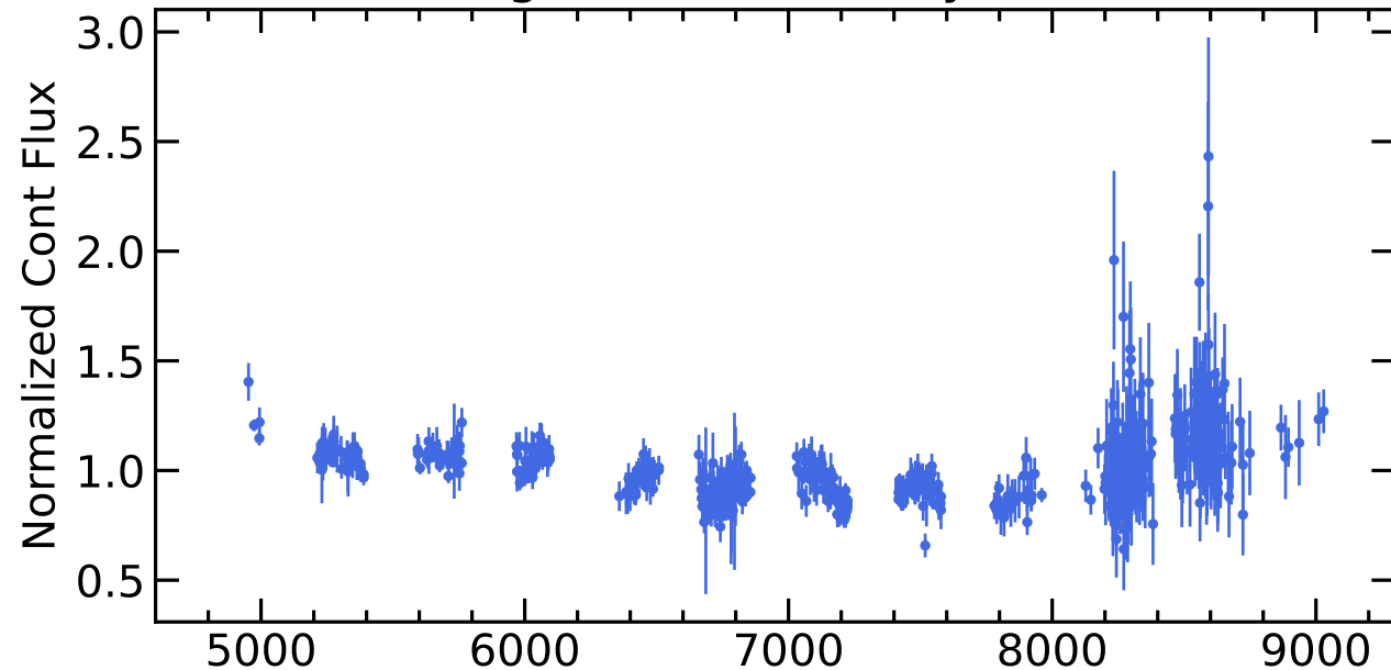
RM438 Light Curves (w/ PyROA model)
