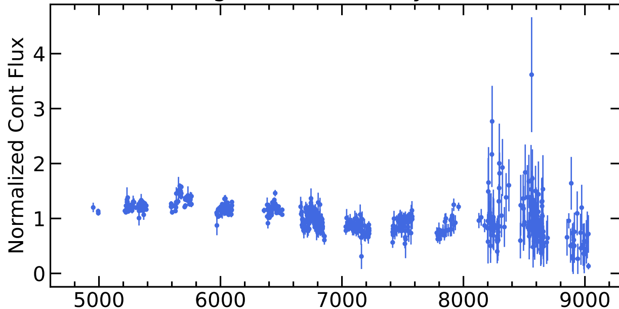
RM439 Light Curves (w/ PyROA model)
