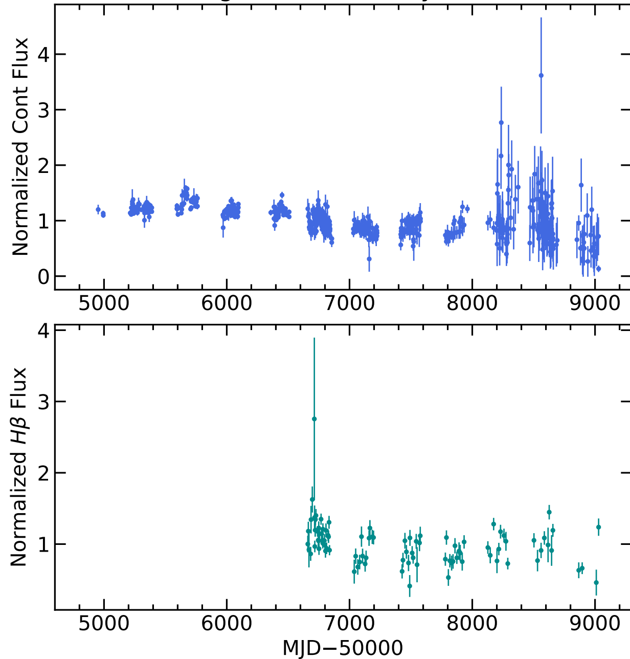
RM439 Light Curves (w/ PyROA model)
