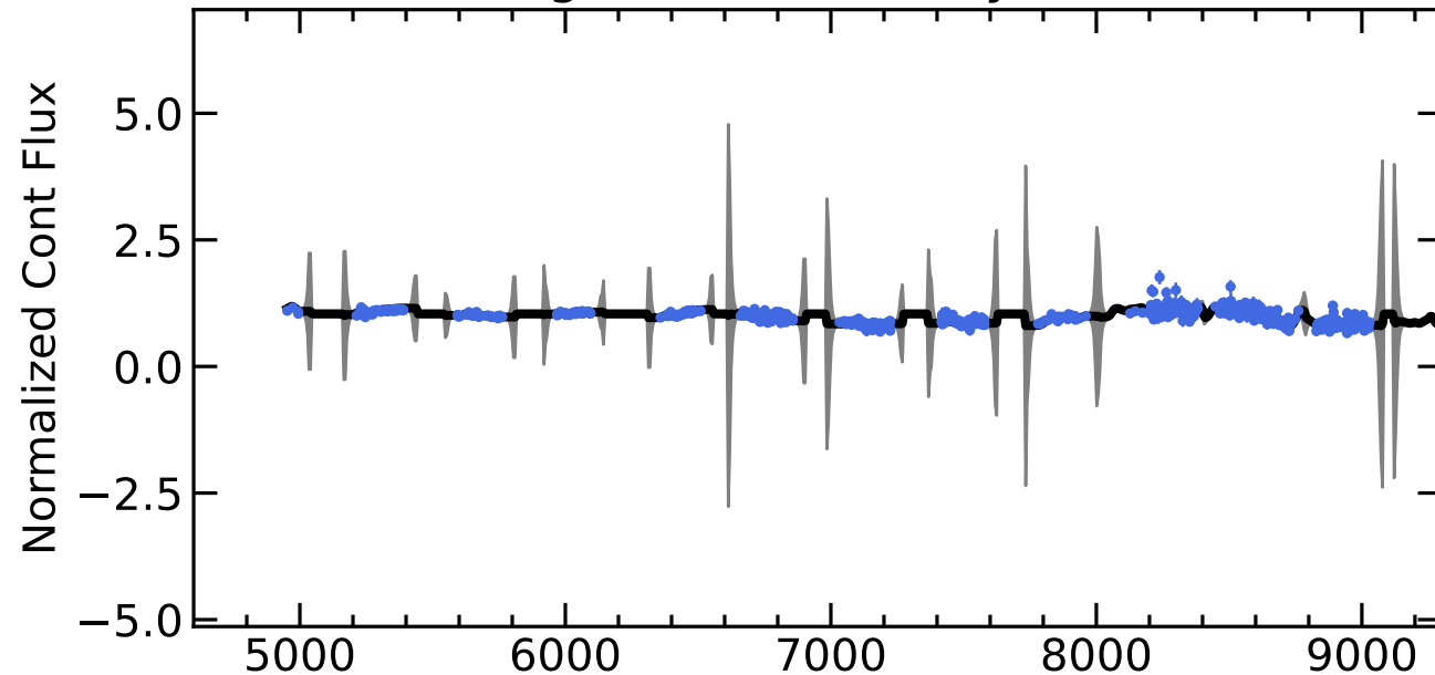
RM441 Light Curves (w/ PyROA model)
