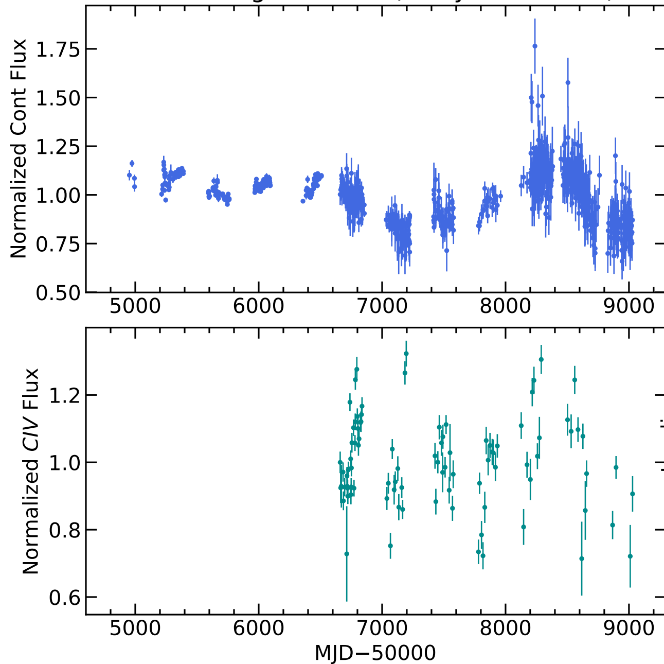
RM441 Light Curves (w/ PyROA model)
