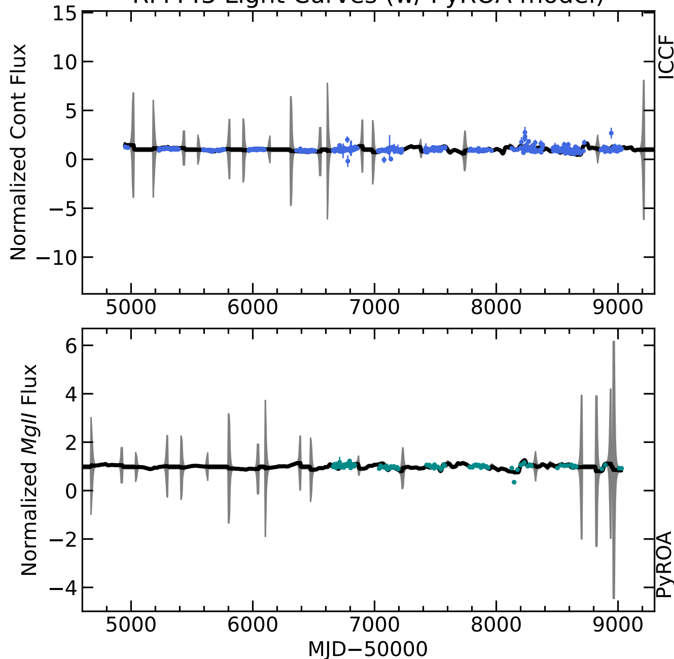
RM443 Light Curves (w/ PyROA model)
