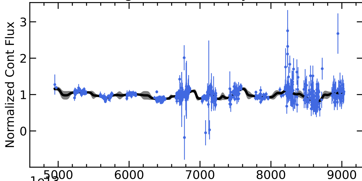
RM443 Light Curves (w/ PyROA model)
