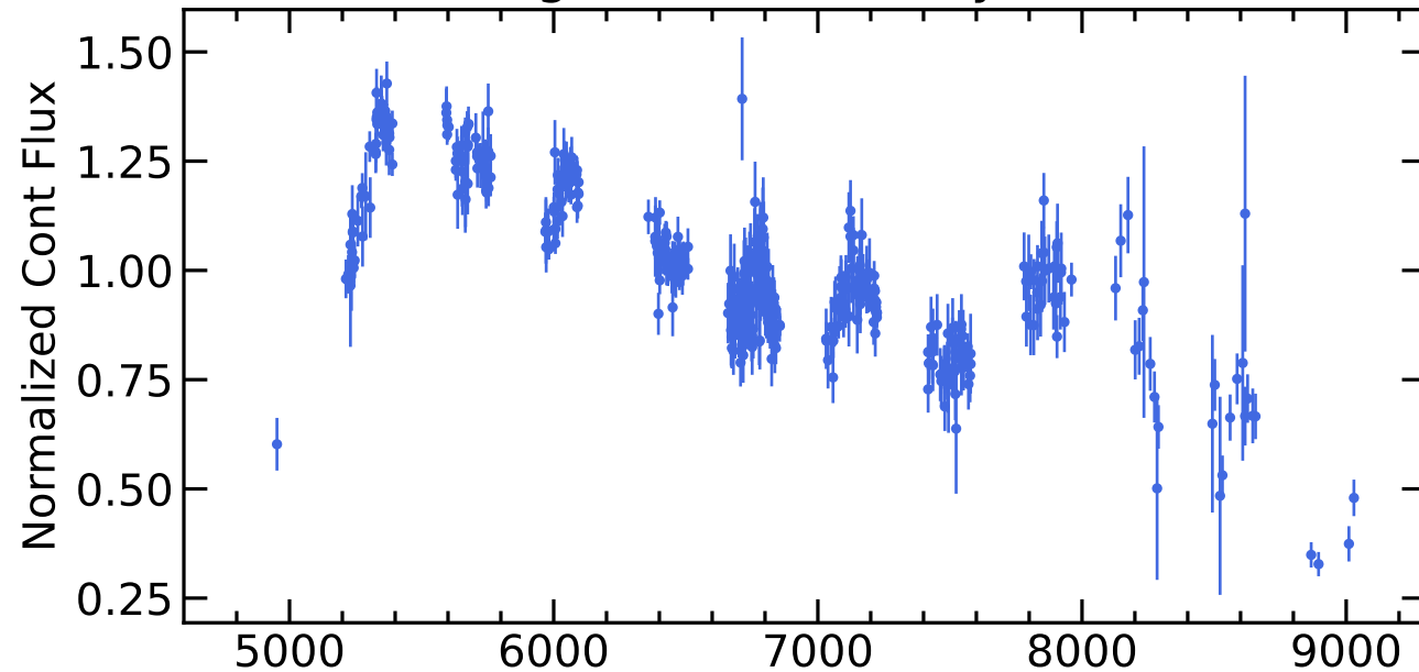
RM444 Light Curves (w/ PyROA model)
