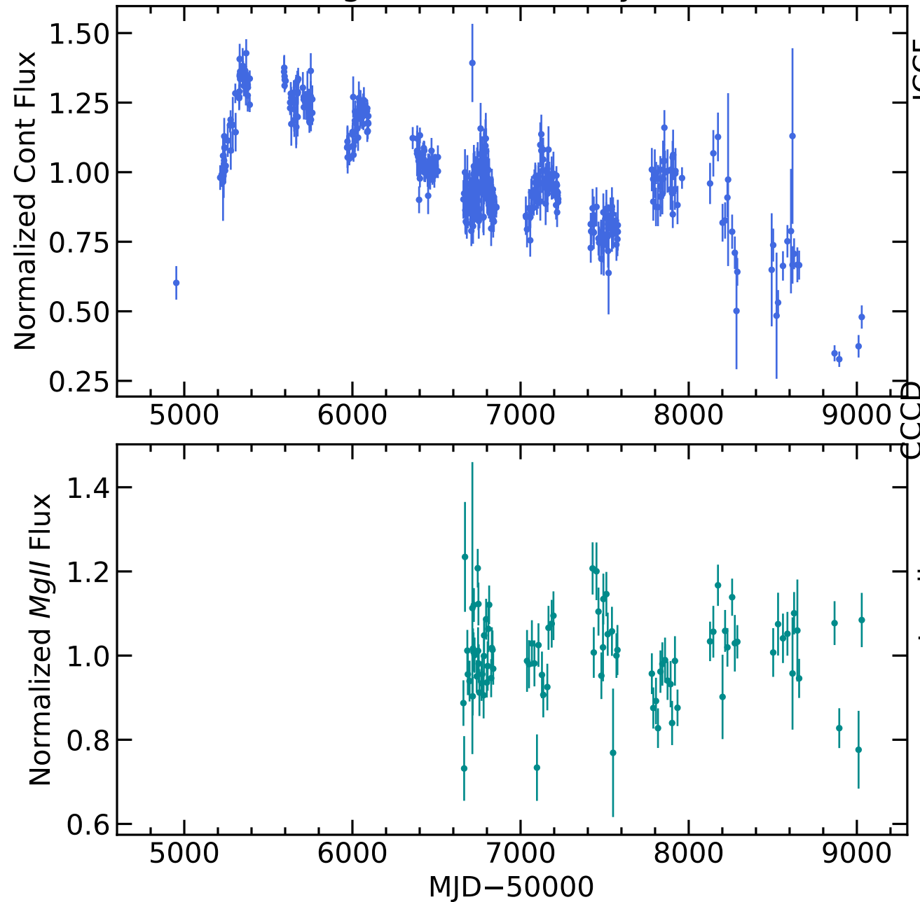
RM444 Light Curves (w/ PyROA model)
