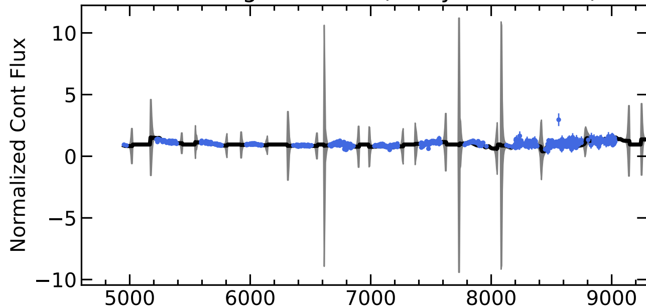
RM445 Light Curves (w/ PyROA model)
