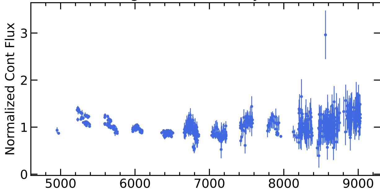
RM445 Light Curves (w/ PyROA model)
