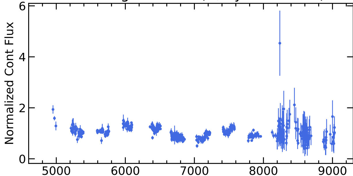
RM446 Light Curves (w/ PyROA model)
