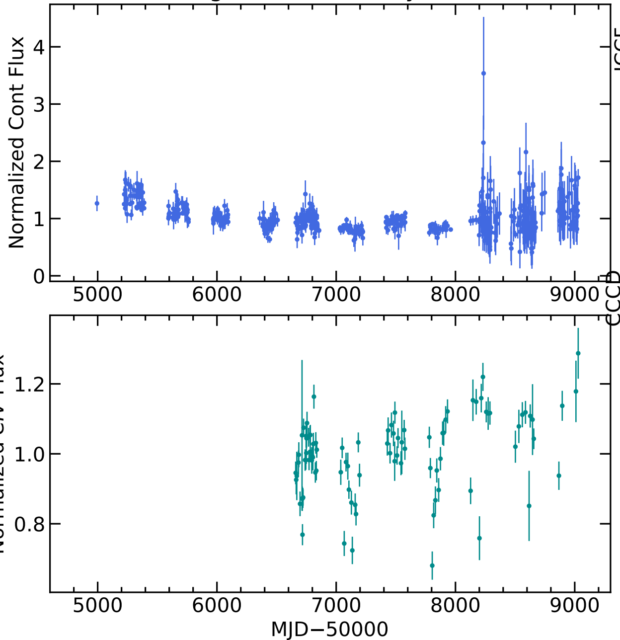
RM447 Light Curves (w/ PyROA model)
