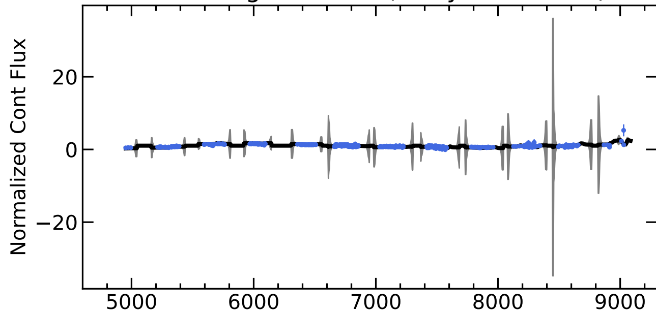
RM448 Light Curves (w/ PyROA model)
