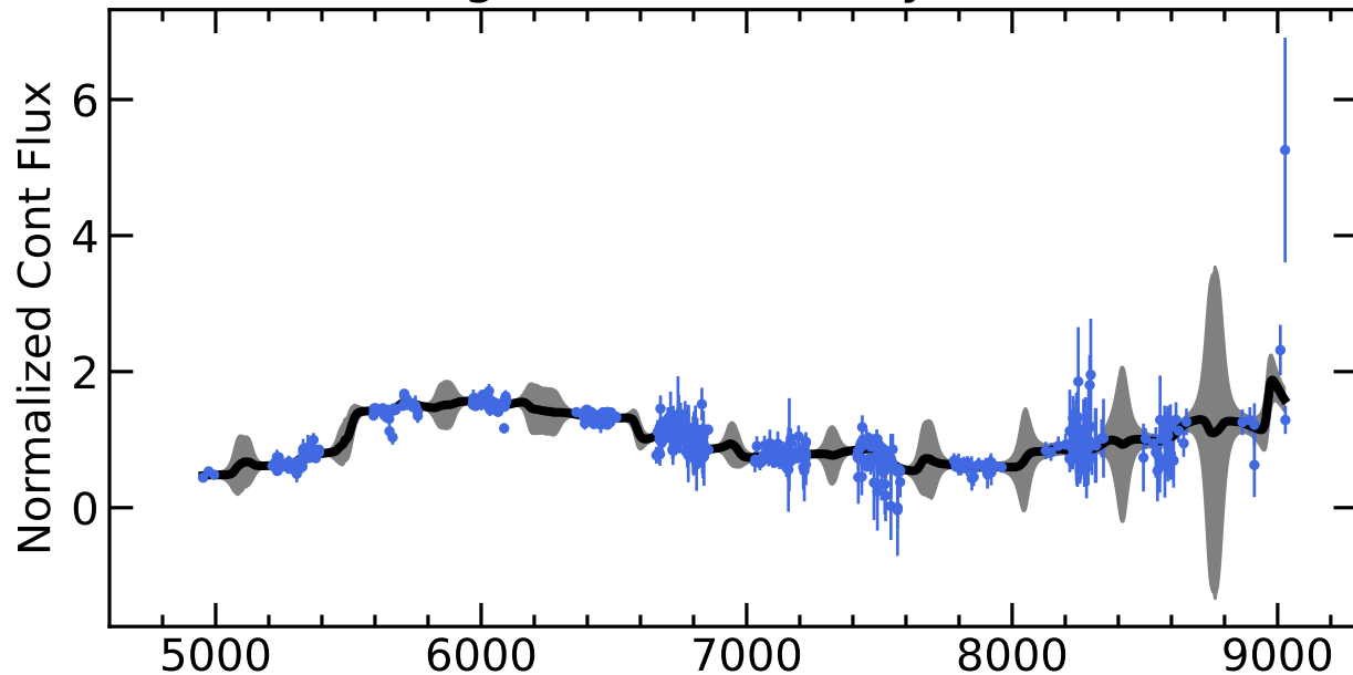
RM448 Light Curves (w/ PyROA model)
