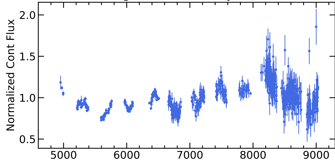
RM449 Light Curves (w/ PyROA model)
