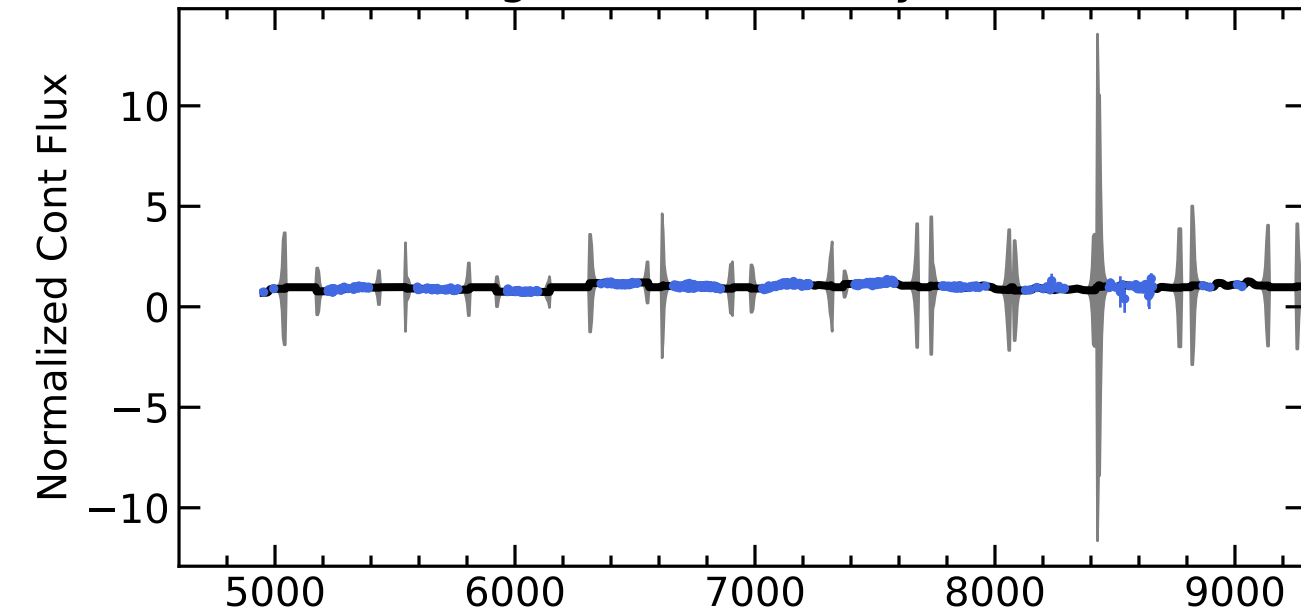
RM450 Light Curves (w/ PyROA model)
