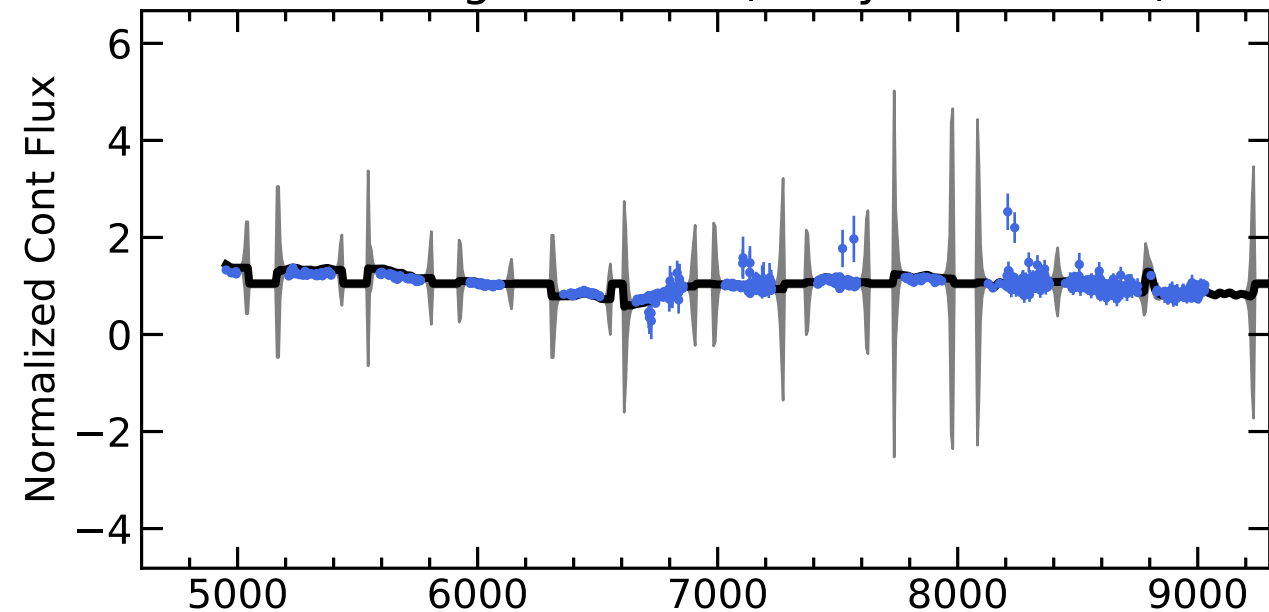
RM451 Light Curves (w/ PyROA model)
