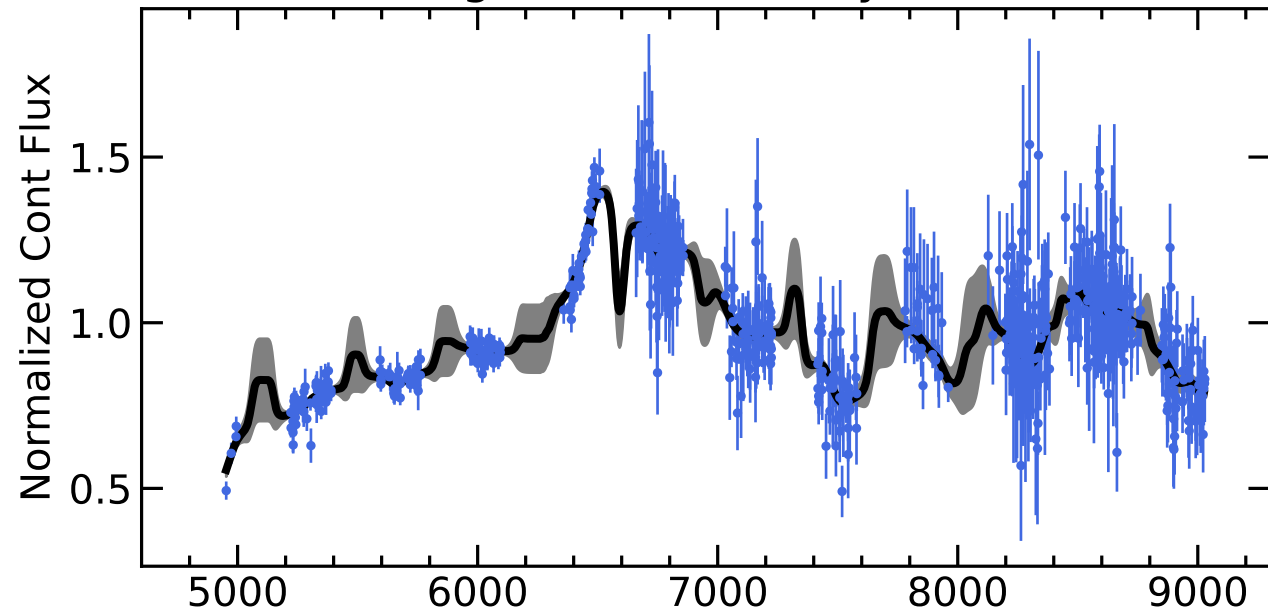
RM452 Light Curves (w/ PyROA model)
