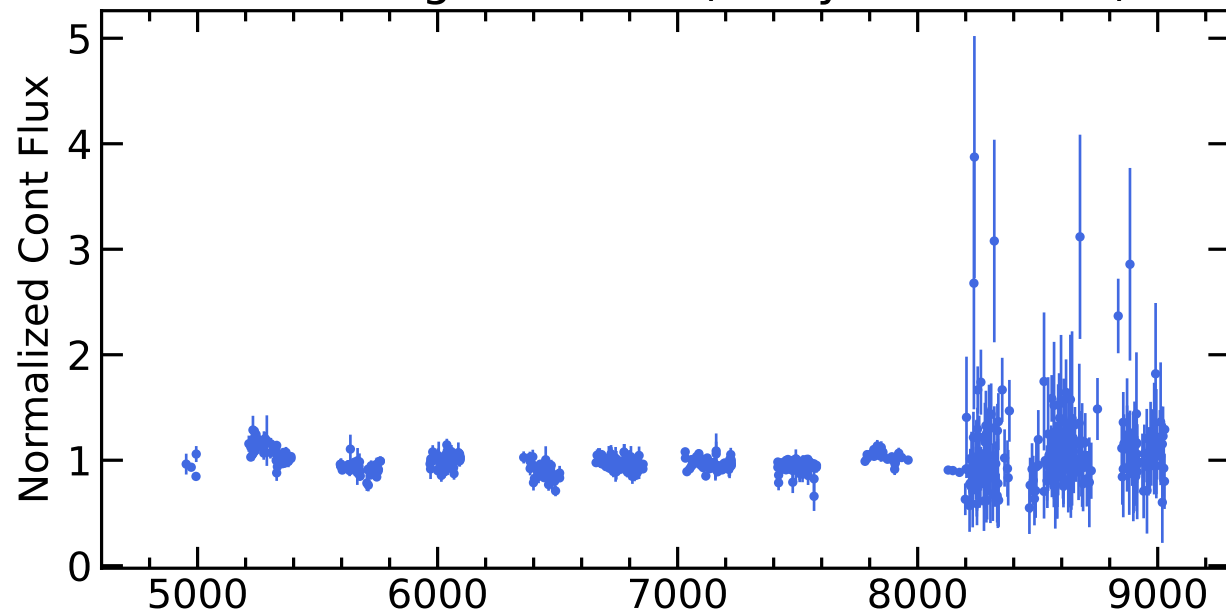
RM453 Light Curves (w/ PyROA model)
