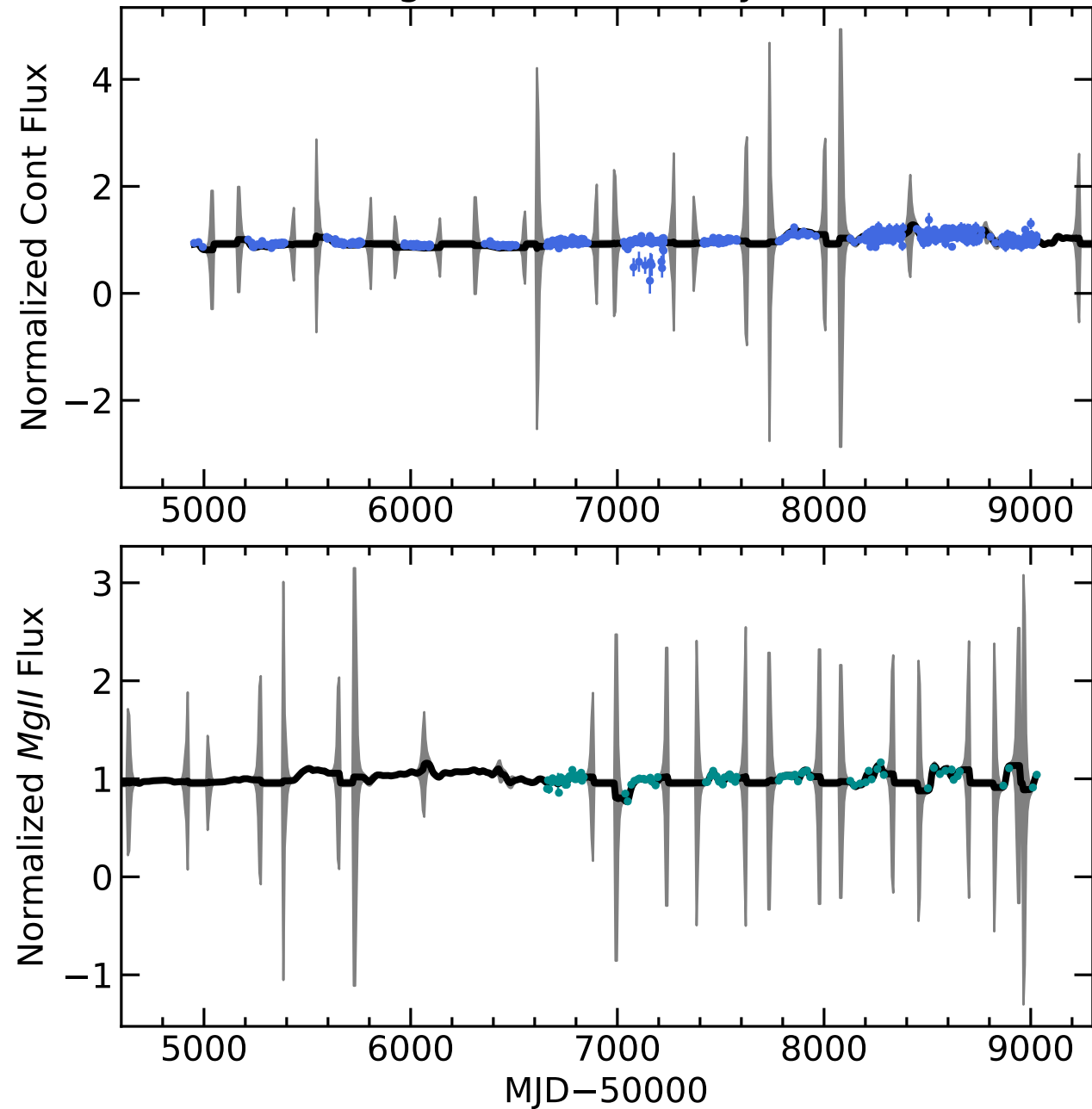
RM454 Light Curves (w/ PyROA model)
