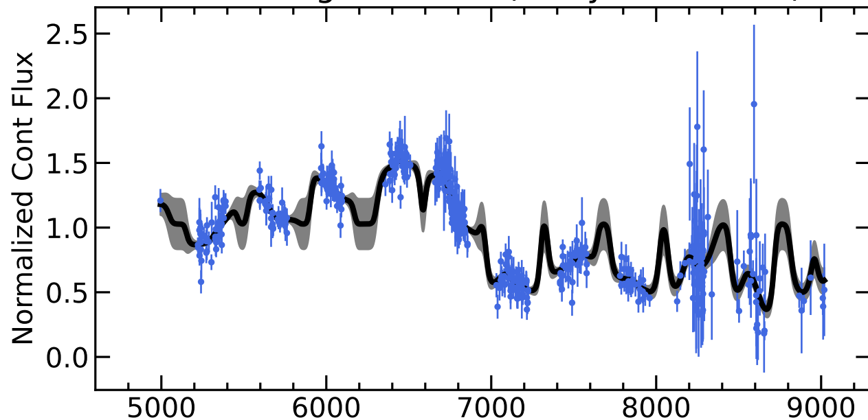
RM455 Light Curves (w/ PyROA model)
