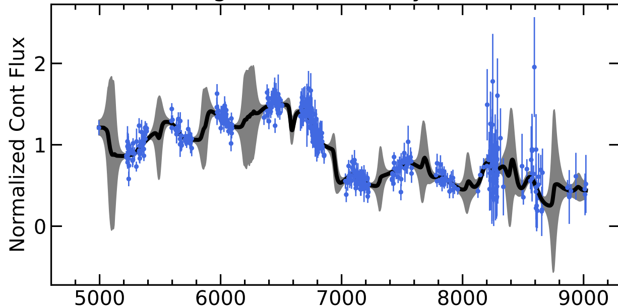
RM455 Light Curves (w/ PyROA model)
