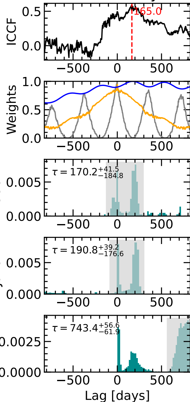
Time Delay
