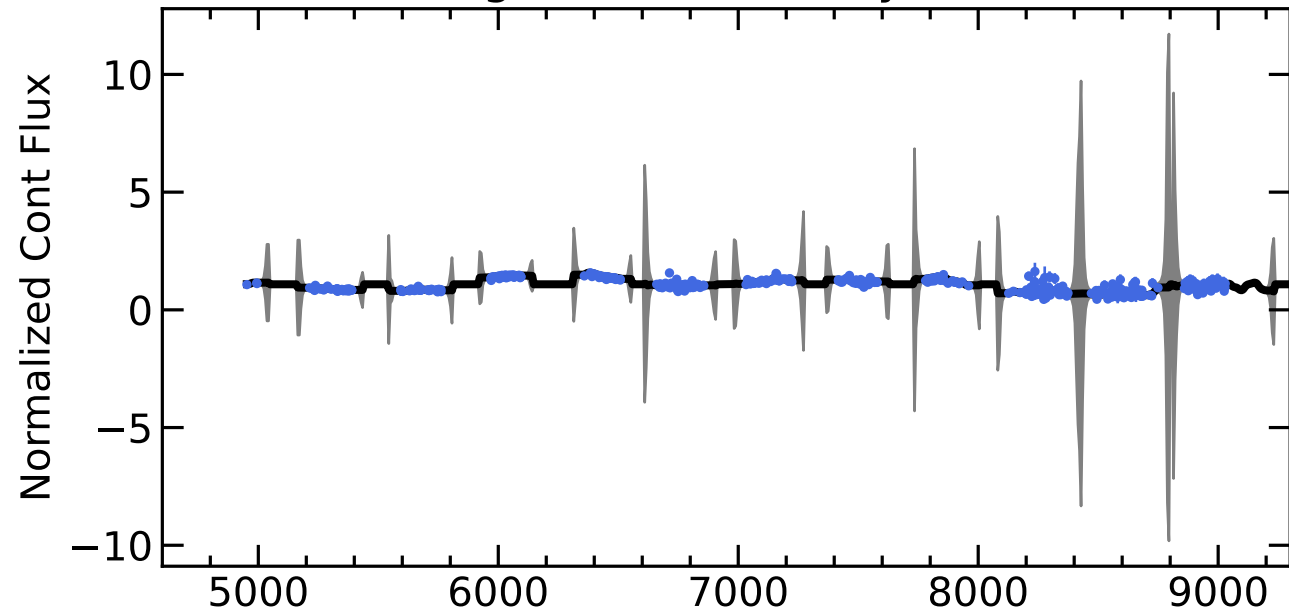
RM456 Light Curves (w/ PyROA model)
