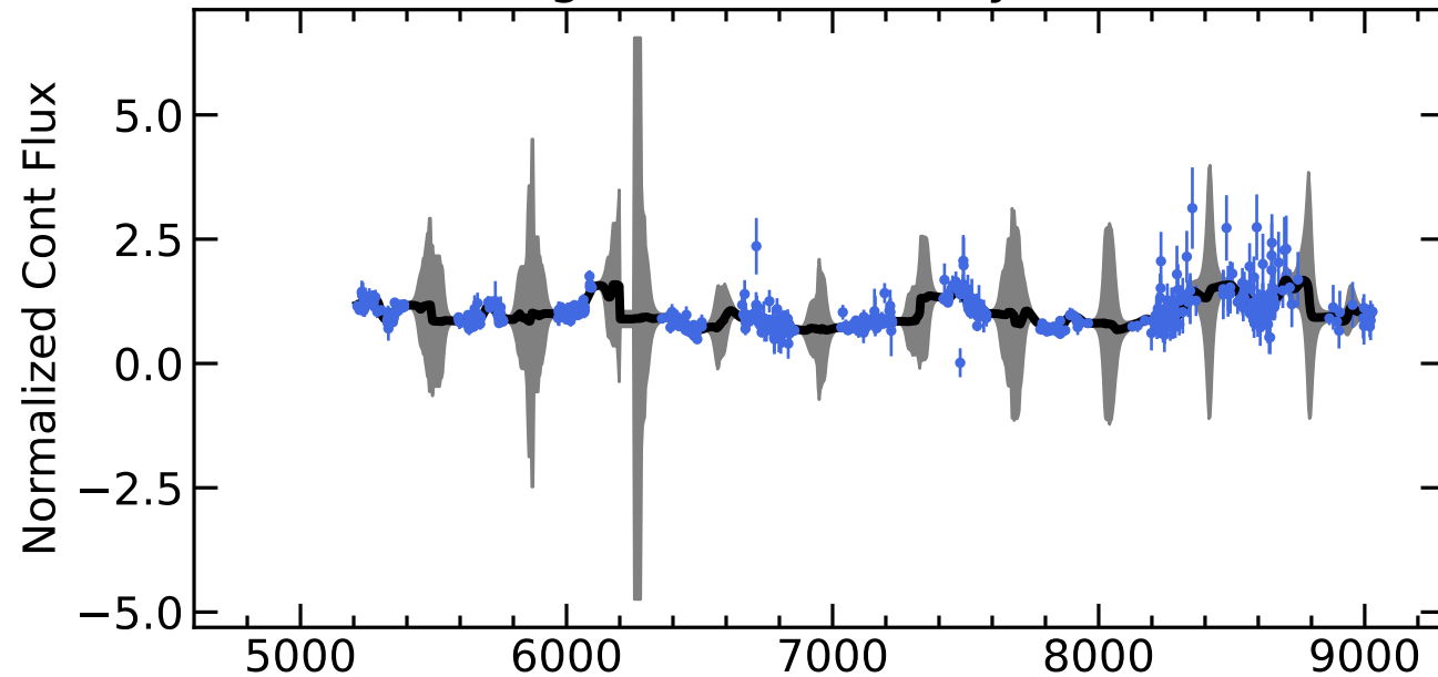
RM457 Light Curves (w/ PyROA model)
