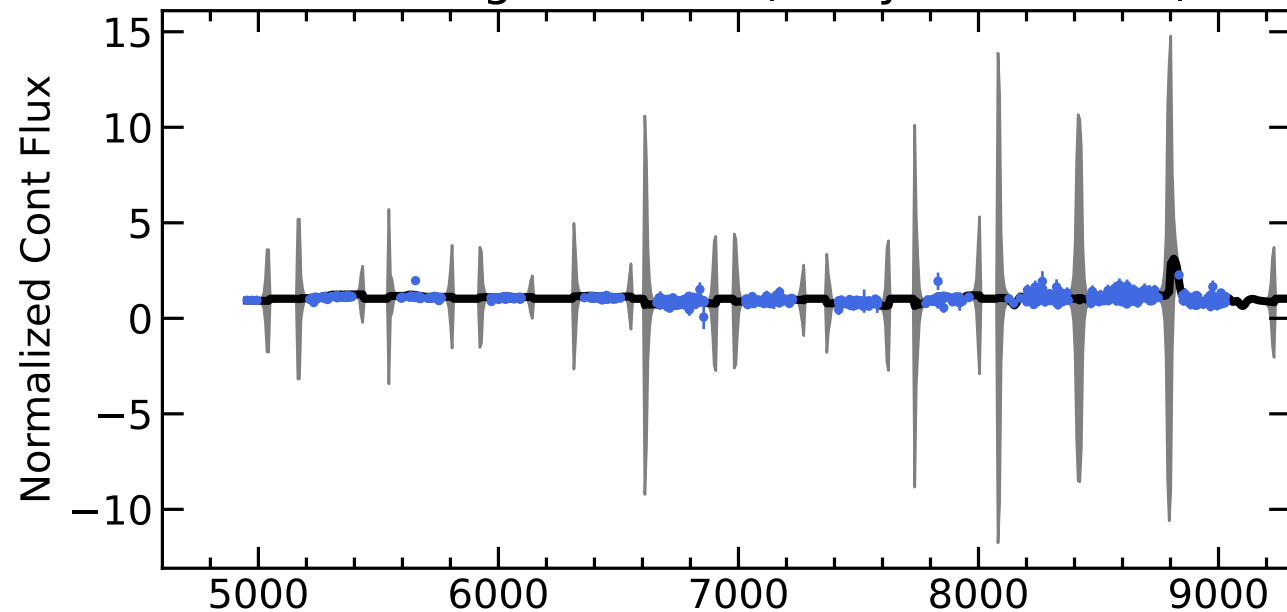
RM458 Light Curves (w/ PyROA model)
