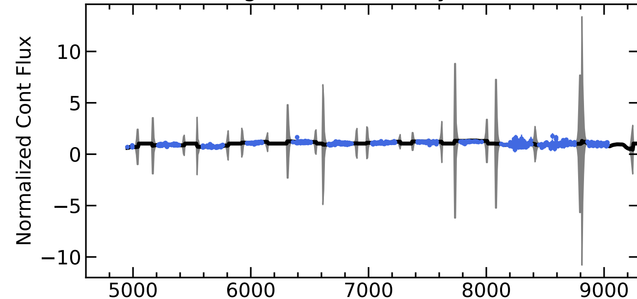
RM461 Light Curves (w/ PyROA model)
