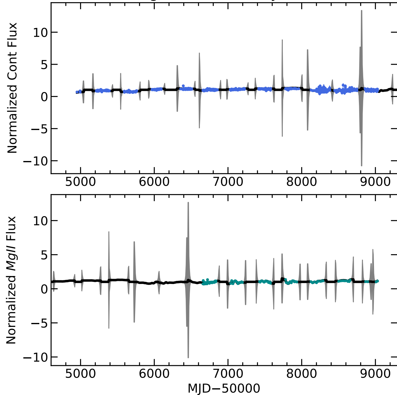
RM461 Light Curves (w/ PyROA model)
