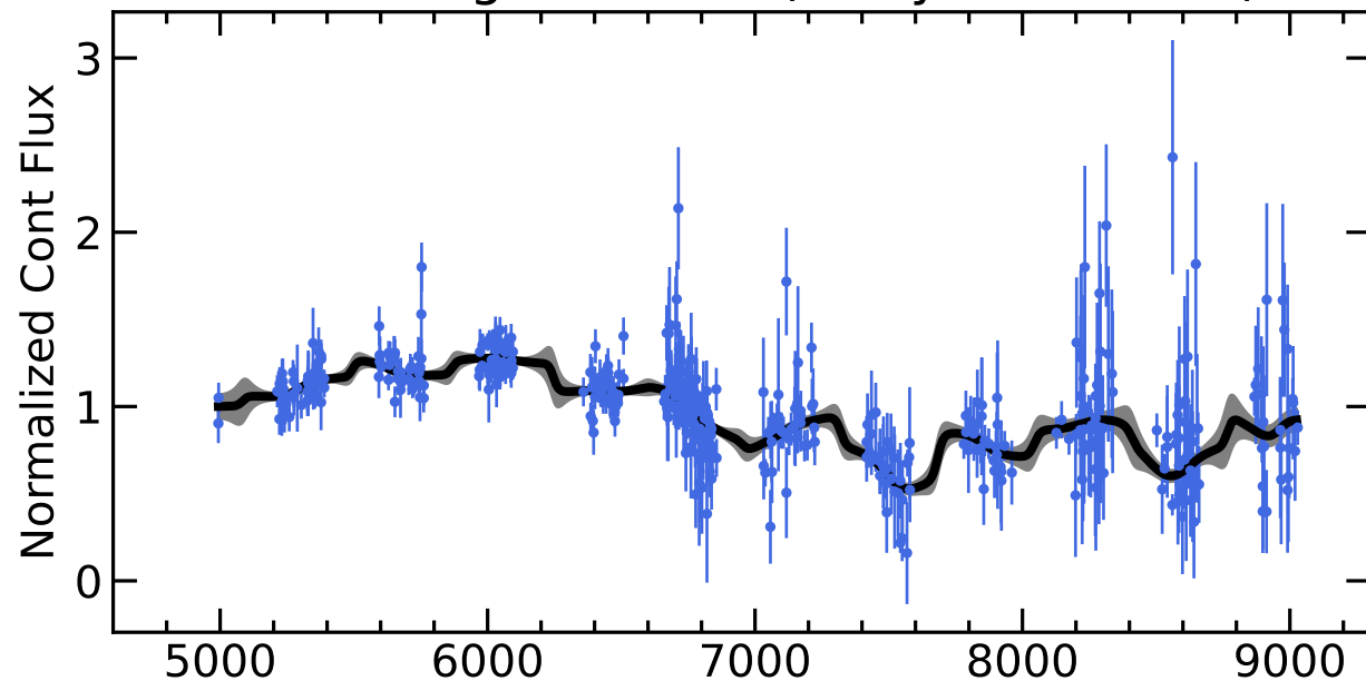
RM462 Light Curves (w/ PyROA model)
