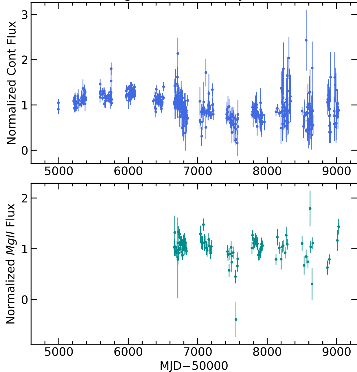
RM462 Light Curves (w/ PyROA model)
