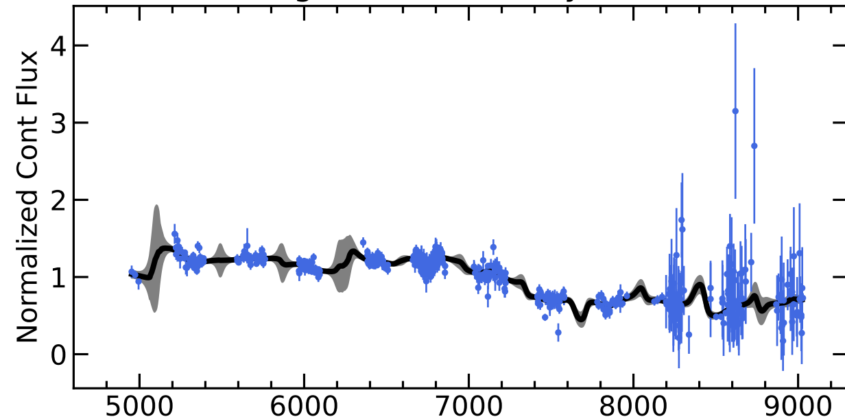
RM463 Light Curves (w/ PyROA model)
