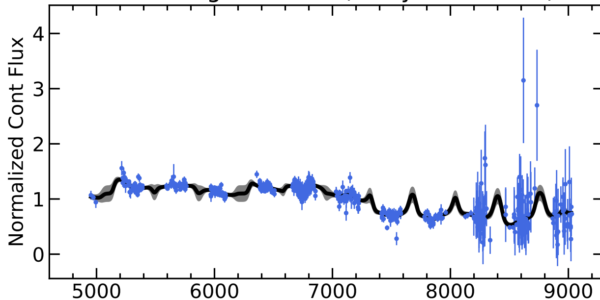
RM463 Light Curves (w/ PyROA model)
