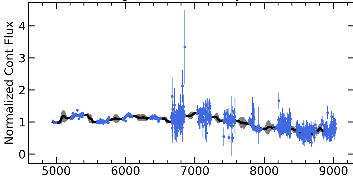
RM464 Light Curves (w/ PyROA model)
