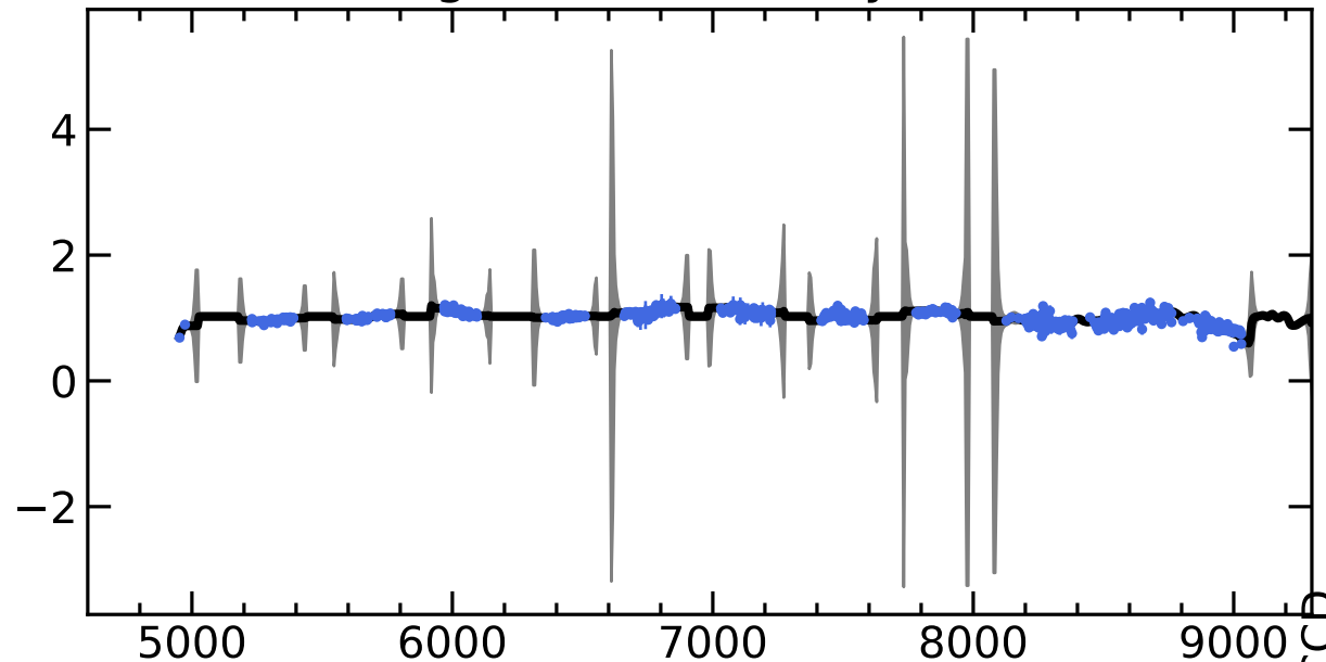
RM465 Light Curves (w/ PyROA model)
