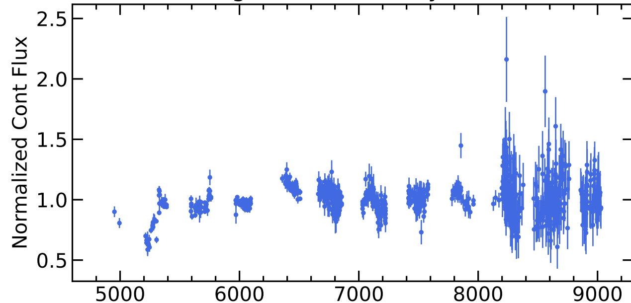
RM466 Light Curves (w/ PyROA model)
