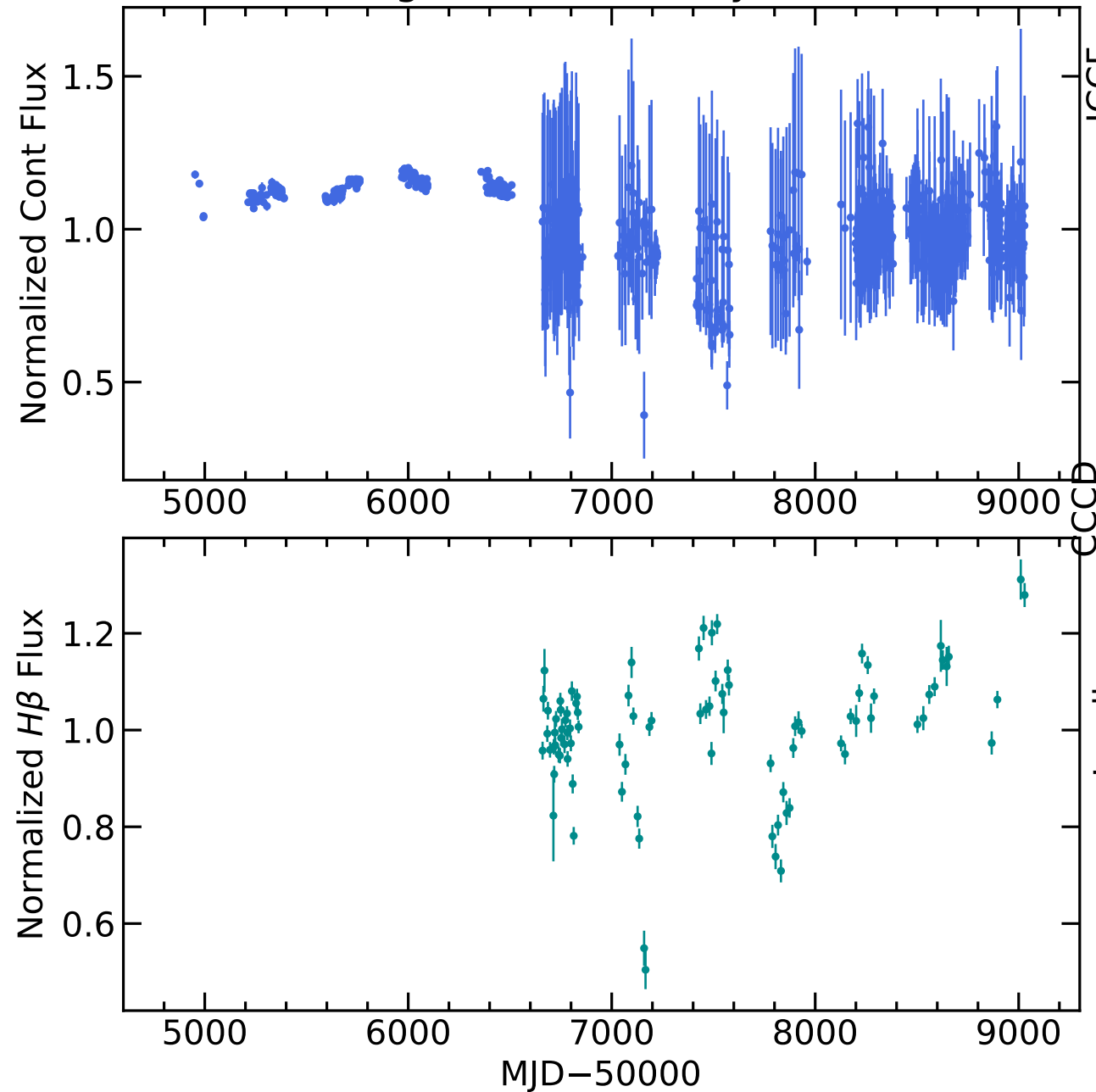
RM469 Light Curves (w/ PyROA model)
