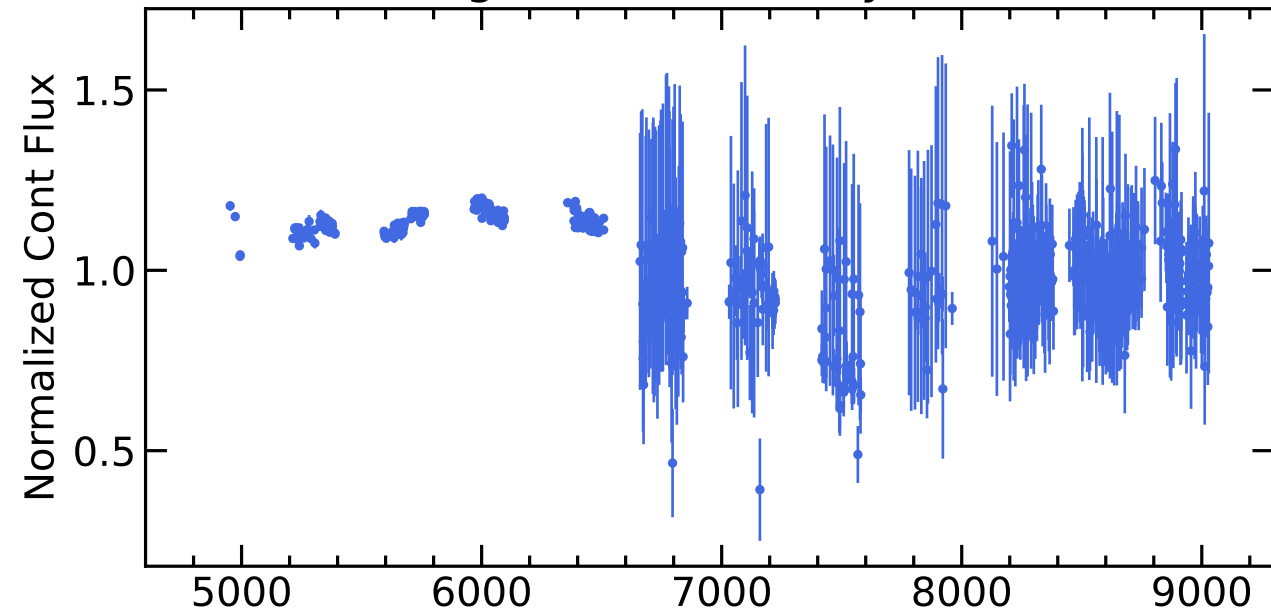
RM469 Light Curves (w/ PyROA model)
