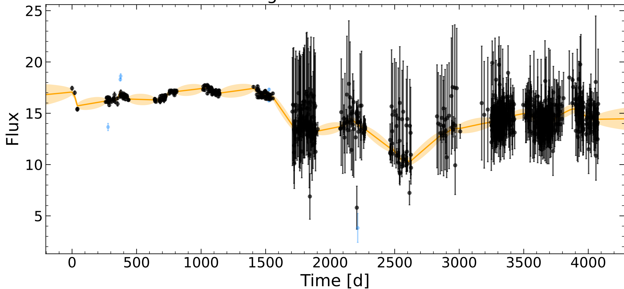
Light Curve of cont
